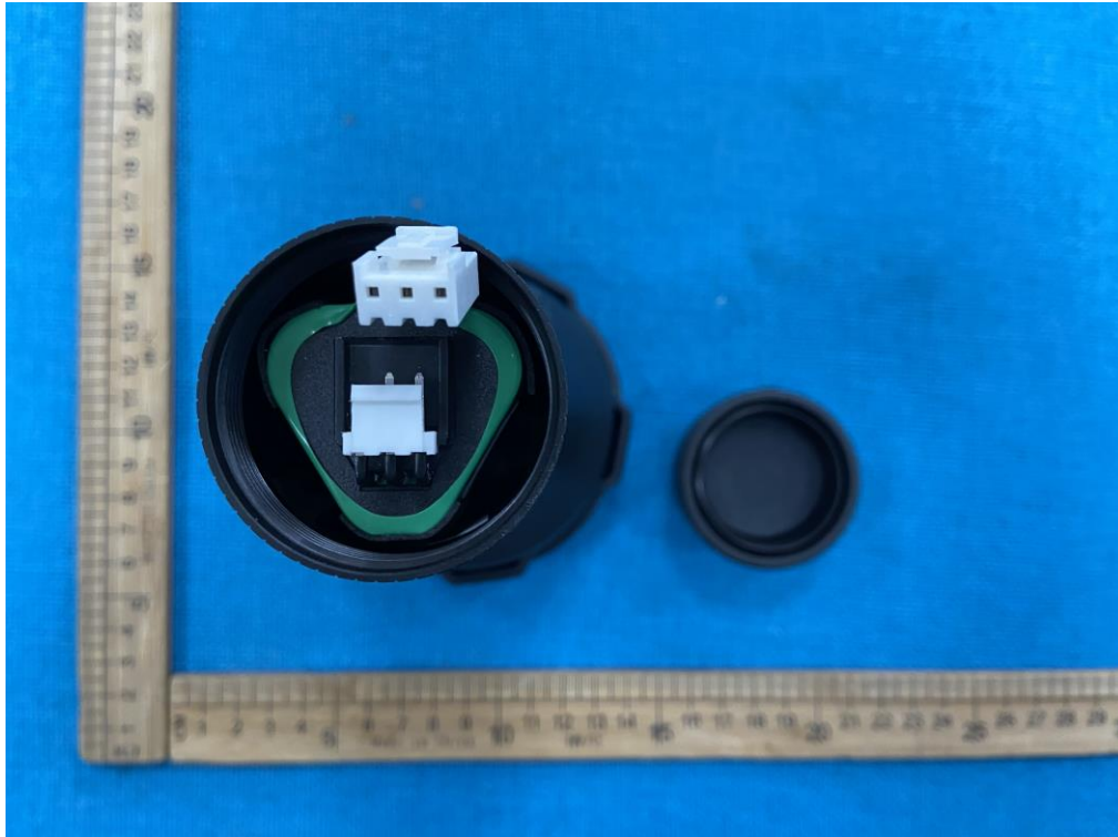
Figure 15. Internal view of unit
