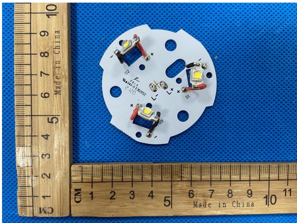
Figure 8. Top view of LED PCB
