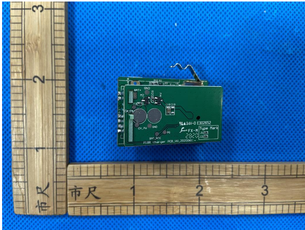
Figure 11. Bottom view of Control board PCB
