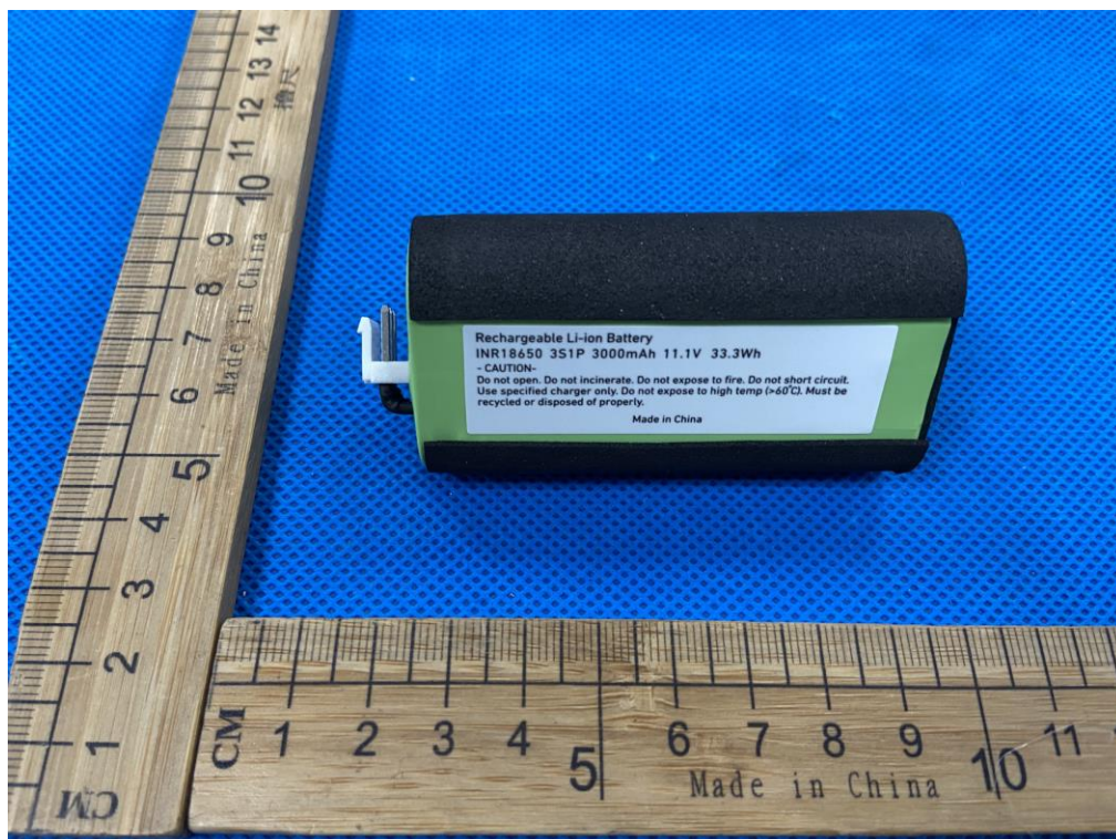
Figure 12. Battery view of unit
