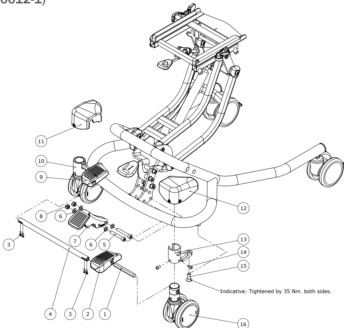
Item numbers for Foot operated central brake kit, size 1, 2 and 3, gas and power (890012-1)
