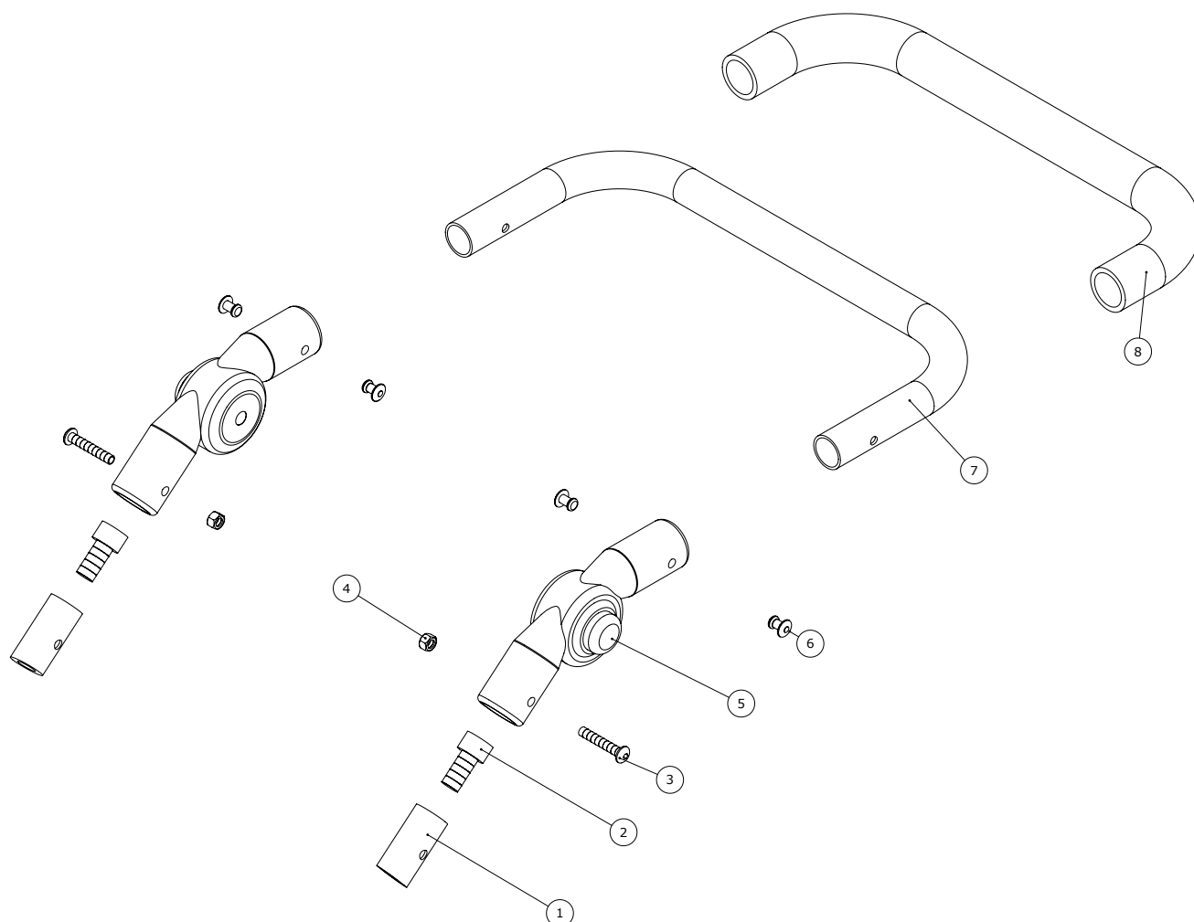
Item numbers for Angle adjustable push brace (95147)
