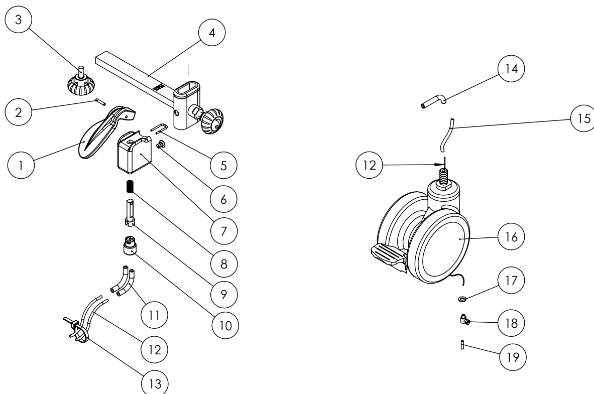
Item numbers for Hand operated central brake kit for retrofitting (890011-3, 890011-4)
