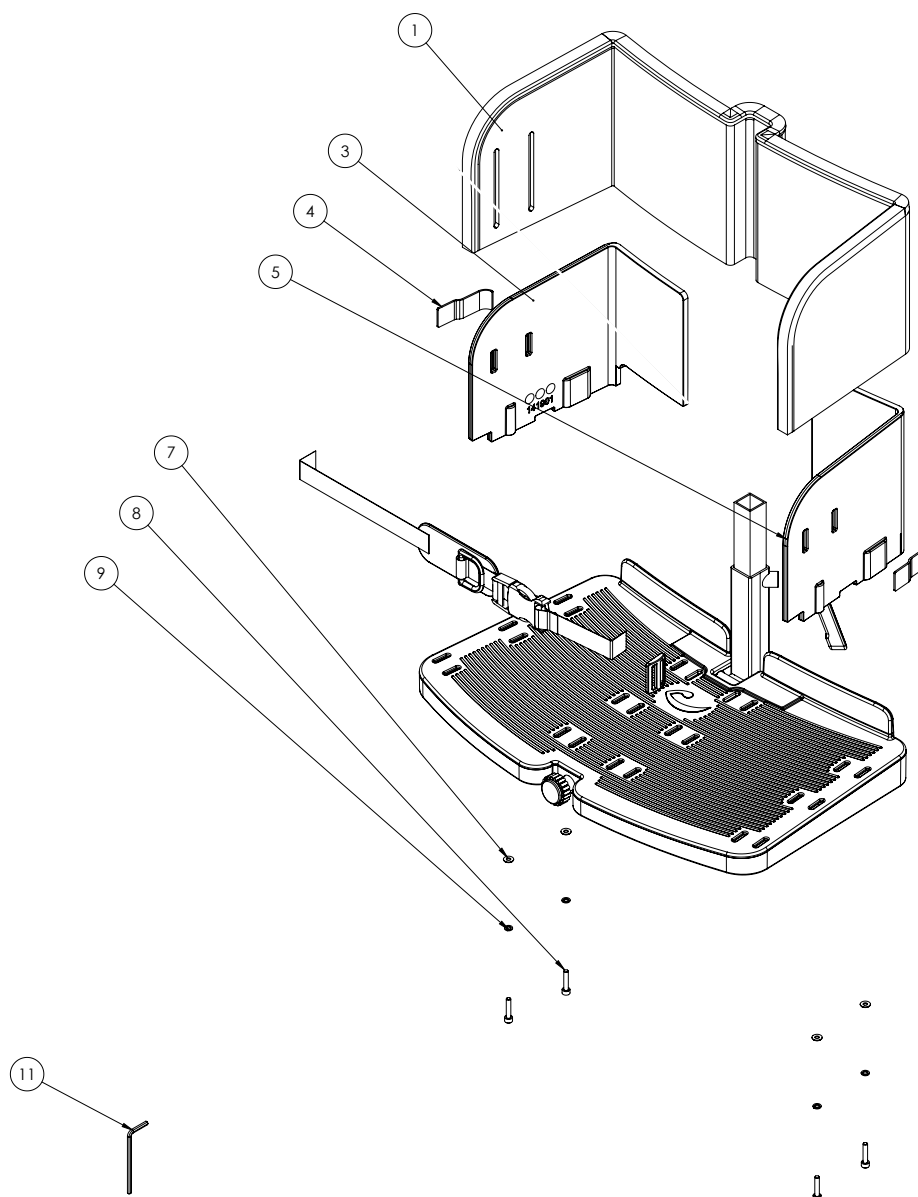
Item numbers for Foot box kit - plate corners and padding for foot plate (95145-1BOX, 95145-2BOX, 95145-3BOX)
