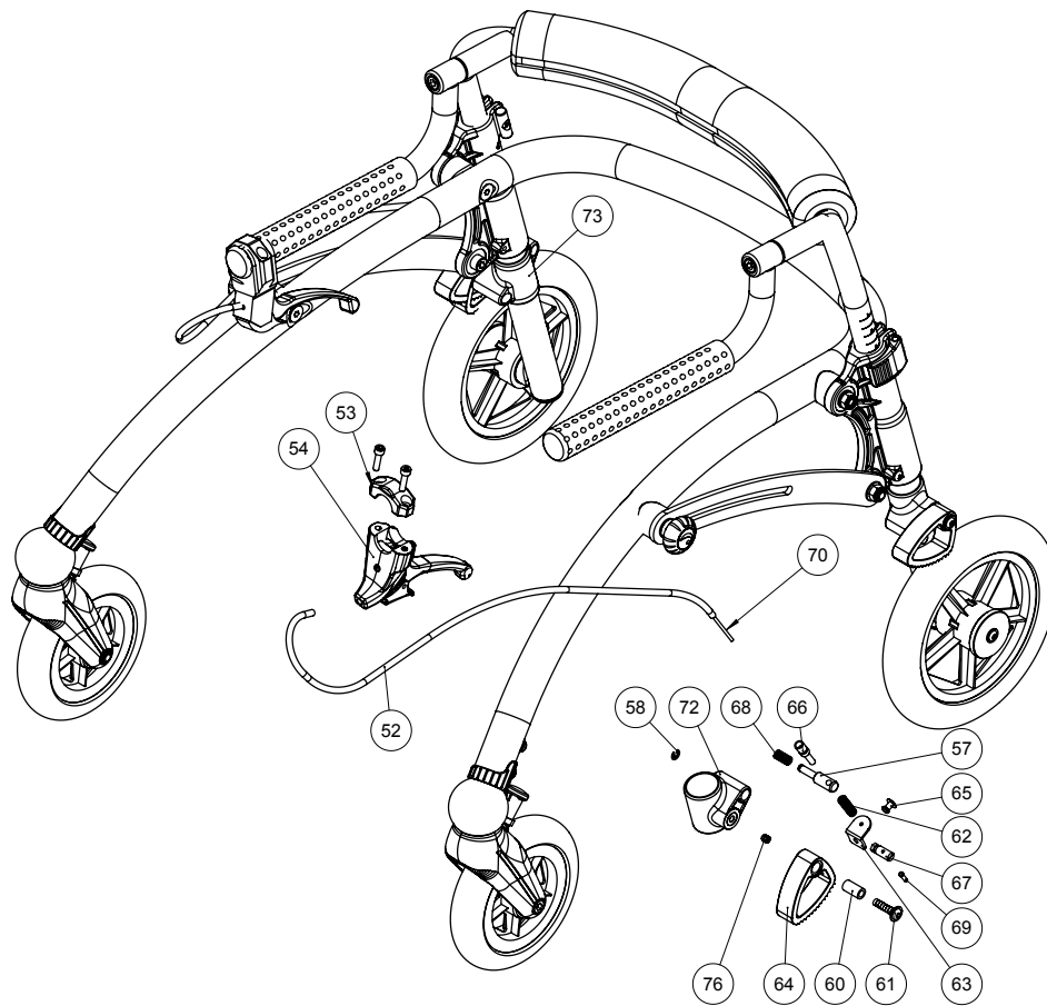
Item numbers for Decelerating hand brake kit- for size 1-2 (86834-DEC)
