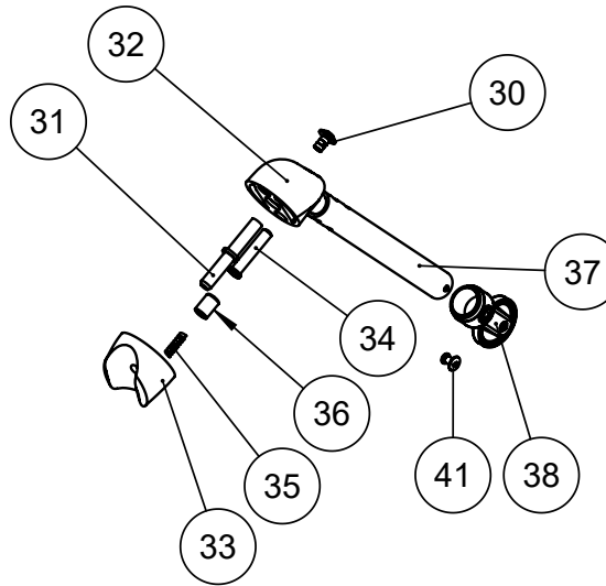
Item numbers for Anti-tip device, swing away - for size 0-2 (86815)
