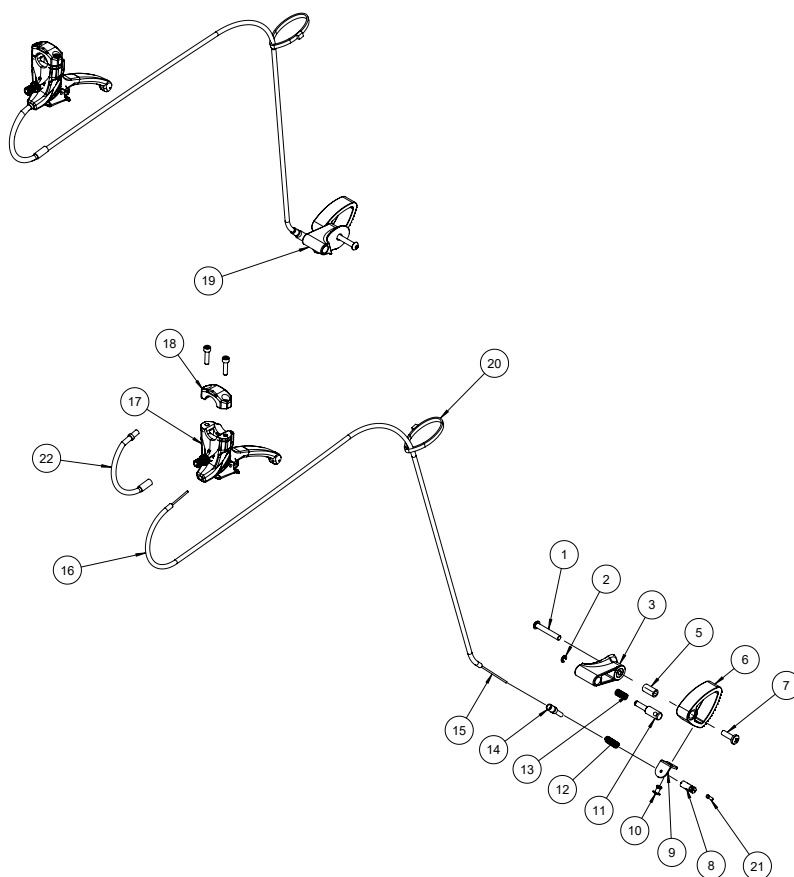
Item numbers for Decelerating hand brake kit- for size 3 (86873-DEC)
