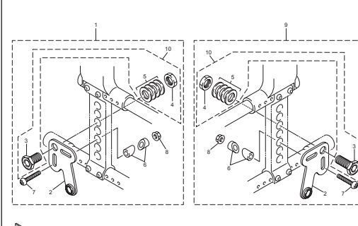
17. Axle sleeve and bracket..... P.47
