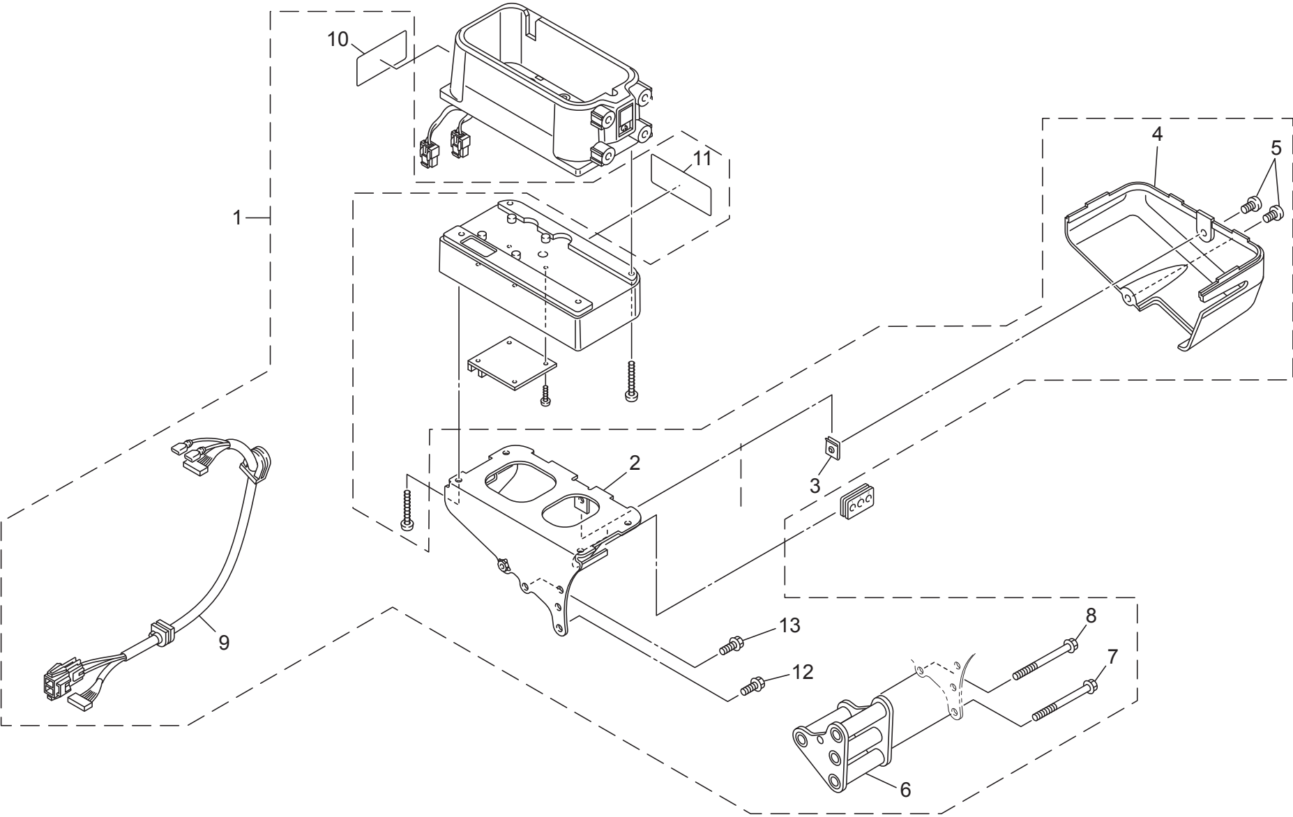
FIG. 15 Battery seat (2)
