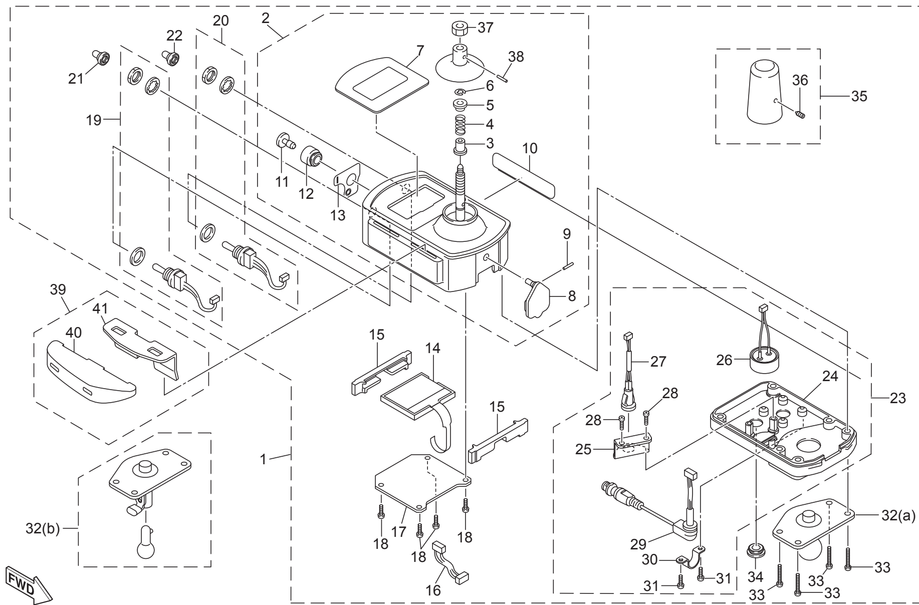
FIG. 3 Joystick controller unit
